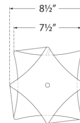
Bottom View
